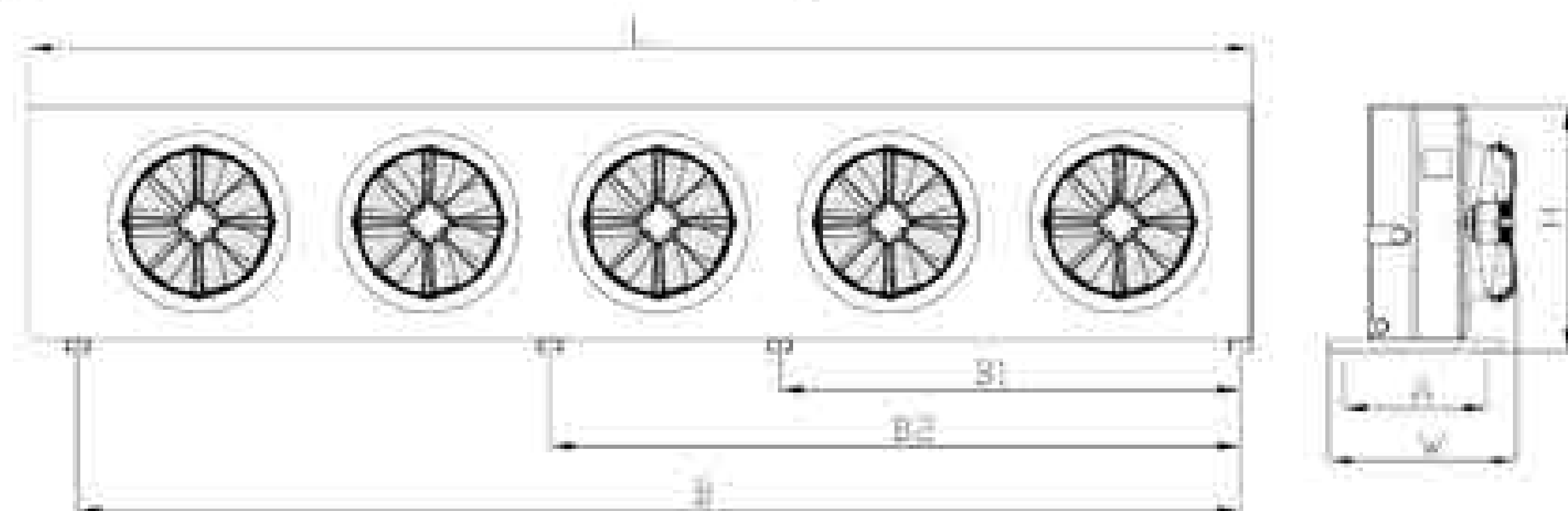
图形A (单排风机) Drawing A (Single row fan)
