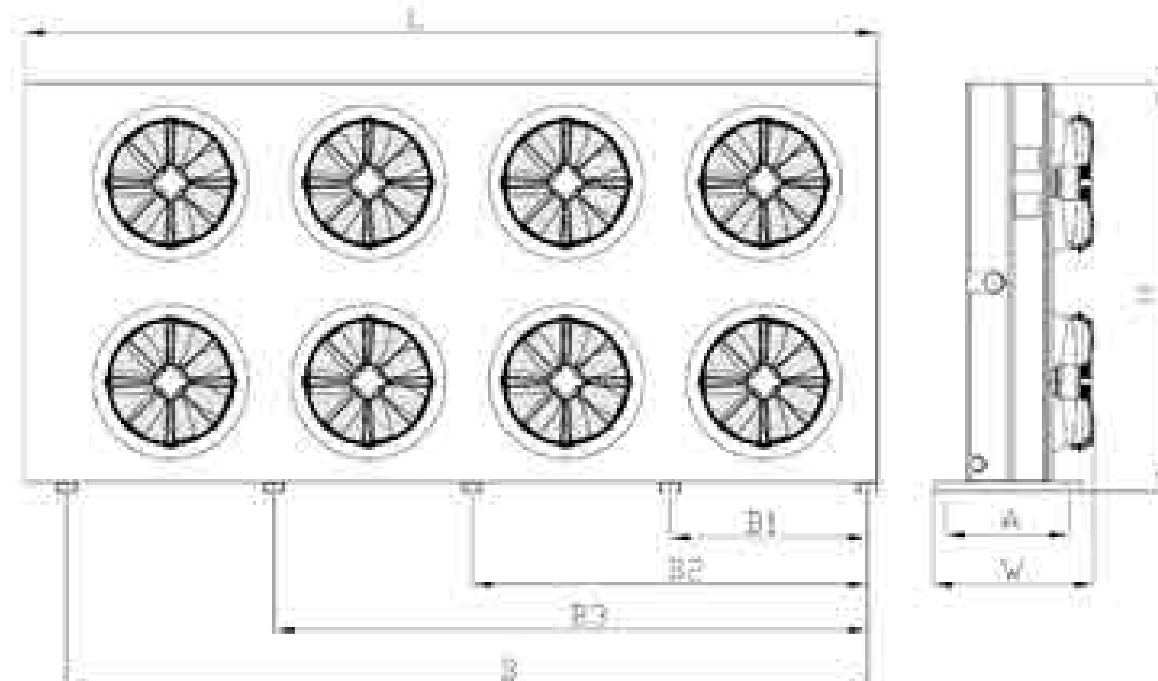
图形B (单排风机) Drawing B (Double row fan)
